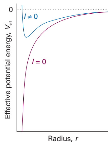
Fig. 10.2 The effective potential energy of an electron in the hydrogen atom. When the electron has zero orbital angular momentum, the effective potential energy is the Coulombic potential energy. When the electron has nonzero orbital angular momentum, the centrifugal effect gives rise to a positive contribution that is very large close to the nucleus. We can expect the l = 0 and l \neq 0 wavefunctions to be very different near the nucleus.
