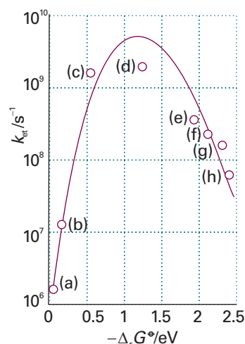
Fig. 24.29 Variation of \log k_{et} with -\Delta_r G^\circ for a series of compounds with the structures given in (1). Kinetic measurements were conducted in 2-methyltetrahydrofuran and at 296 K. The distance between donor (the reduced biphenyl group) and the acceptor is constant for all compounds in the series because the molecular linker remains the same. Each acceptor has a characteristic standard reduction potential, so it follows that the standard Gibbs energy for the electron transfer process is different for each compound in the series. The line is a fit to a version of eqn 24.84 and the maximum of the parabola occurs at -\Delta_r G^\circ = \lambda = 1.2 \text{ eV} = 1.2 \times 10^2 \text{ kJ mol}^{-1} . (Reproduced with permission from J.R. Miller, L.T. Calcaterra, and G.L. Closs, J. Amer. Chem. Soc. 106 , 3047 (1984).)
