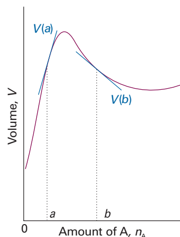
Fig. 5.2 The partial molar volume of a substance is the slope of the variation of the total volume of the sample plotted against the composition. In general, partial molar quantities vary with the composition, as shown by the different slopes at the compositions a and b . Note that the partial molar volume at b is negative: the overall volume of the sample decreases as A is added.
