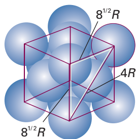
Fig. 20.36 The calculation of the packing fraction of an ccp unit cell.
