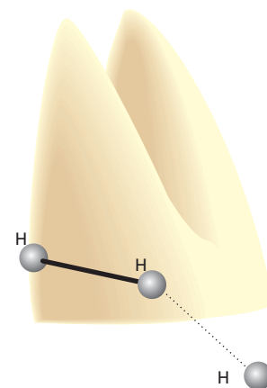
Fig. 24.19 An indication of the anisotropy of the potential energy changes as H_2 with different angles of attack. The collinear attack has the lowest potential barrier to reaction. The surface indicates the potential energy profile along the reaction coordinate for each configuration.
