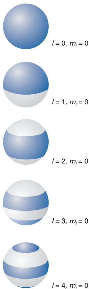
Fig. 9.36 A representation of the wavefunctions of a particle on the surface of a sphere which emphasizes the location of angular nodes: dark and light shading correspond to different signs of the wavefunction. Note that the number of nodes increases as the value of l increases. All these wavefunctions correspond to m_l = 0 ; a path round the vertical z -axis of the sphere does not cut through any nodes.
